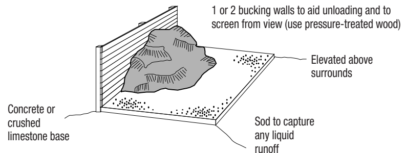
Figure 7. Manure pad slope and drainage. Drain and gutter are recommended in all cases, especially if the manure stack will not be protected from rainfall. Leachate (effluent) must be directed to a storage tank and/or suitable method of disposal.
